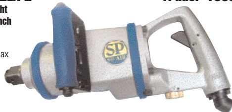
Twin Dog Clutch
